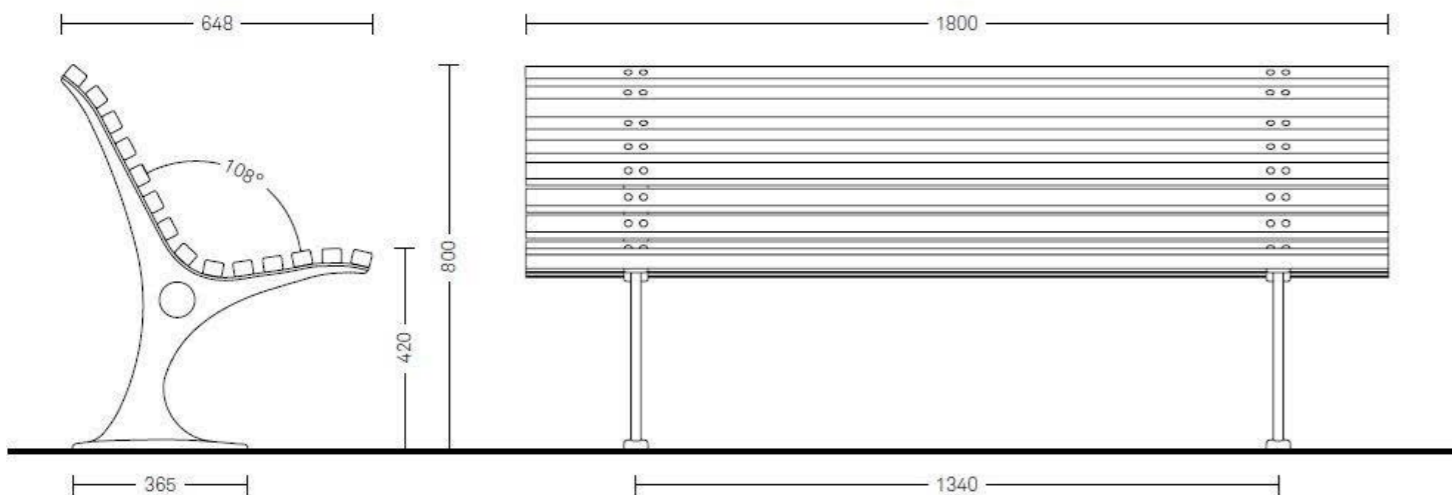
Bench 2147.002 T
