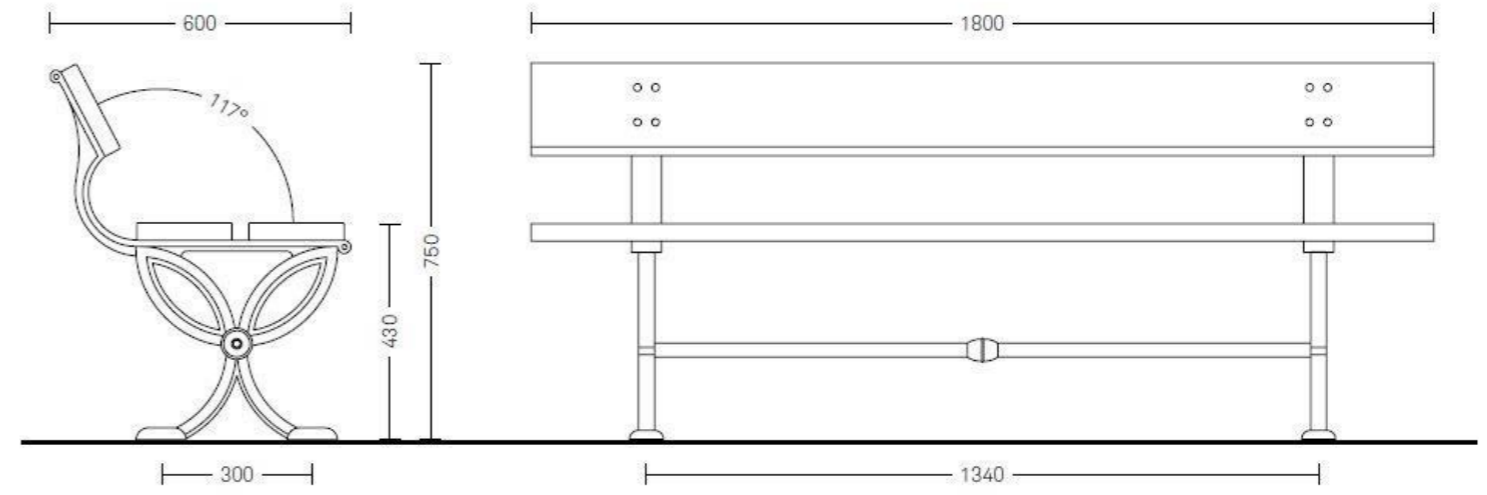
Bench 2170.002.018 M
